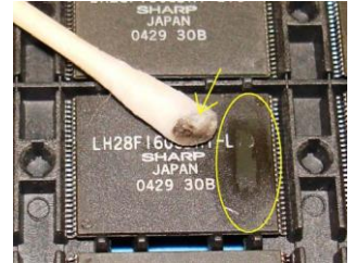
Blacktopped Part
