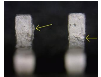
Resoldered Lead
